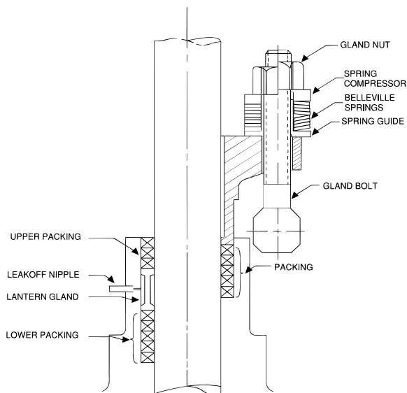
Packing Chamber with Leakoff
