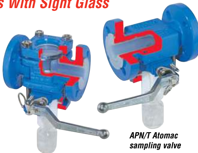
APN/SG Atomac sampling valve with sight glass
