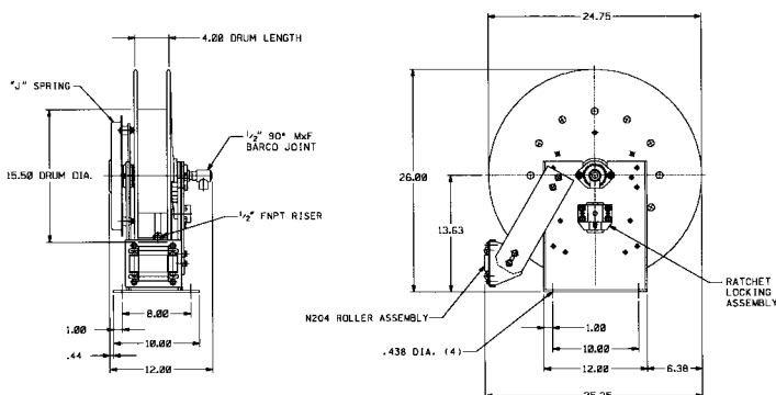
Standard hose reel to be used with our \frac{5}{8} " I.D. hose assembly "R" or "RS" only, maximum length 50 ft.
