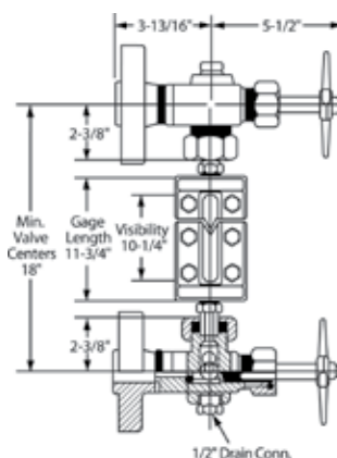
MODEL EFI 2027
