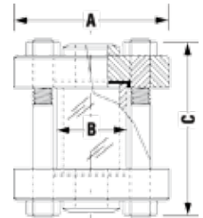
MODEL EFI 17280
