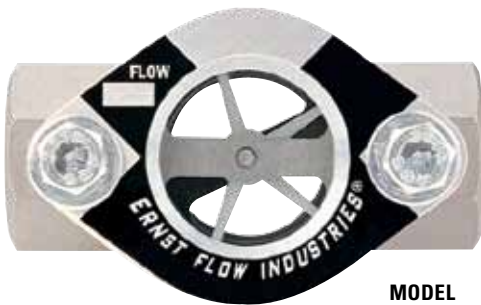
MODEL EFI 1421 Carbon Steel EFI 1431 Bronze EFI 1471 316 Stainless Steel EFI 1481 Ductile Iron
