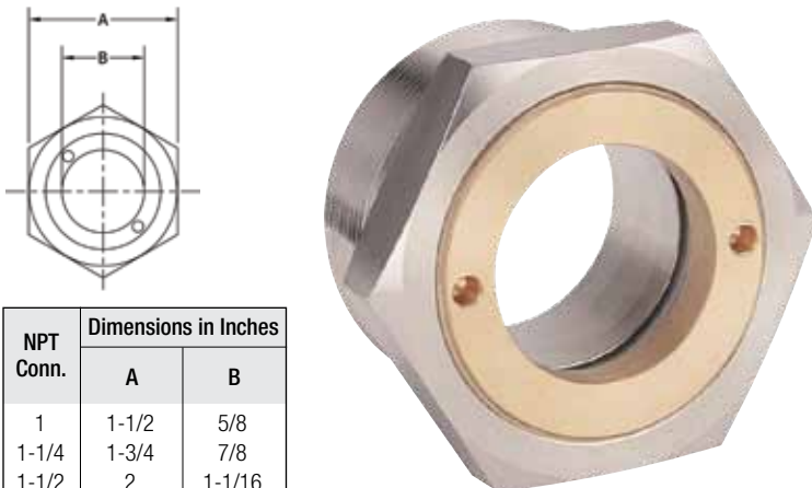
MODEL EFI S5400
