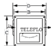
MODEL EFI 815BC (Without Microswitch)
