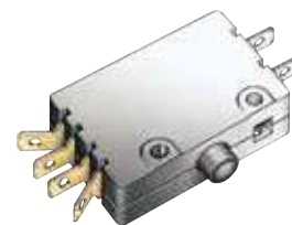
Type 3 (2) DPDT Mechanical 15 amp @ 125 VAC Minimum 50 mA Consult factory for DC voltages
