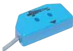
Type E / P1 Sabre Switch (2) SPDT Proximity 1 amp @ 120 VAC, 1 amp @ 24 VDC, 25 Watt Max. Minimum 1 mA
