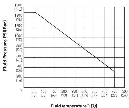
Pressure and Temperature Rating of LE Packing
