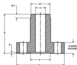
Non-Contoured Nozzle
